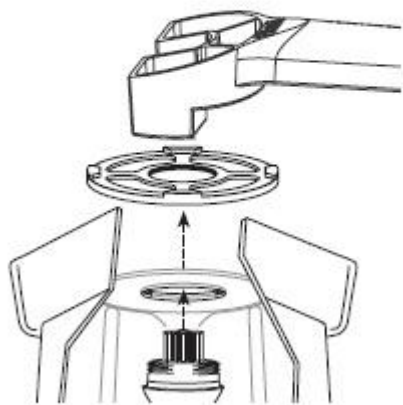
Retainer Nut Wrench in use
